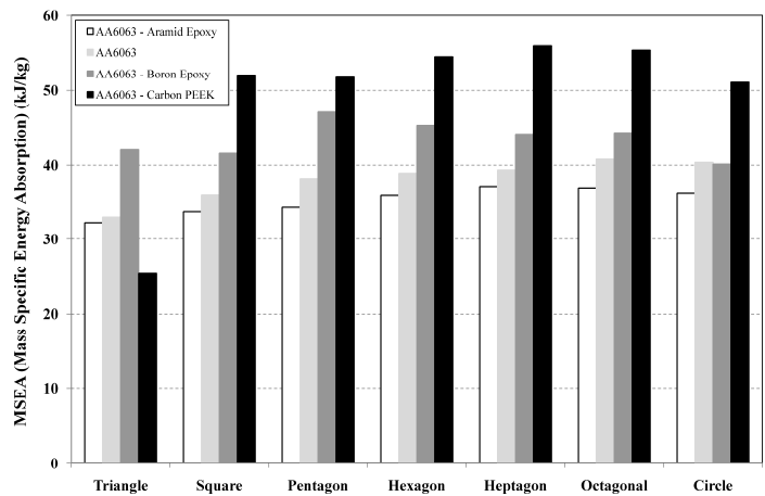
Fig11. Effects of cross-section shape and material properties on the MSEA in hybrid tubes
